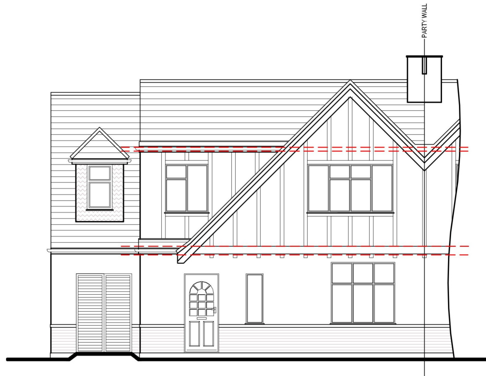
PROPOSED EAST FACING FRONT ELEVATION
