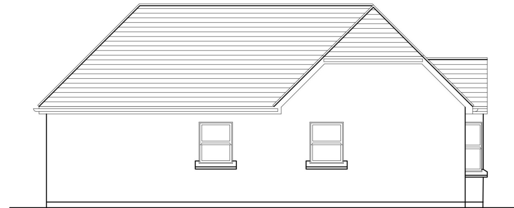
EXISTING SOUTH FACING SIDE ELEVATION
