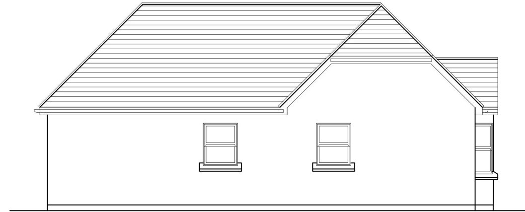
PROPOSED SOUTH FACING SIDE ELEVATION
