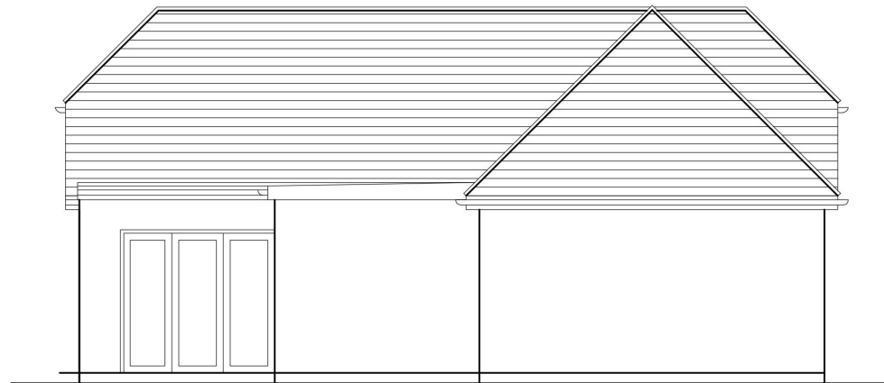
PROPOSED WEST FACING REAR ELEVATION
