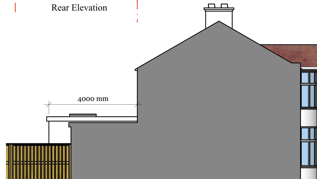
East Elevation
