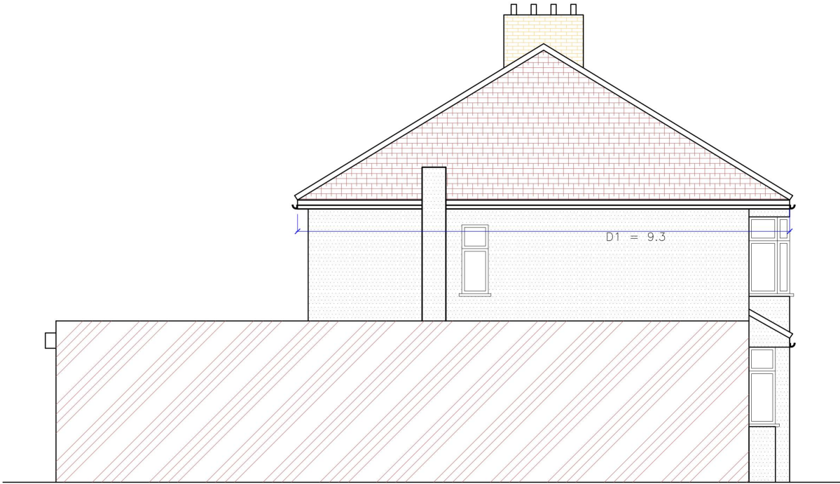
Existing Side Elevation - A
