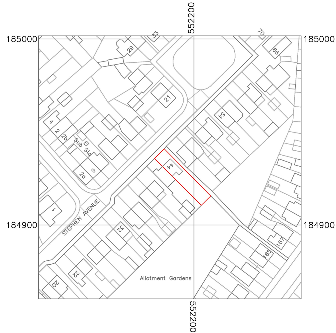
THE LOCATION PLAN 1:1250
