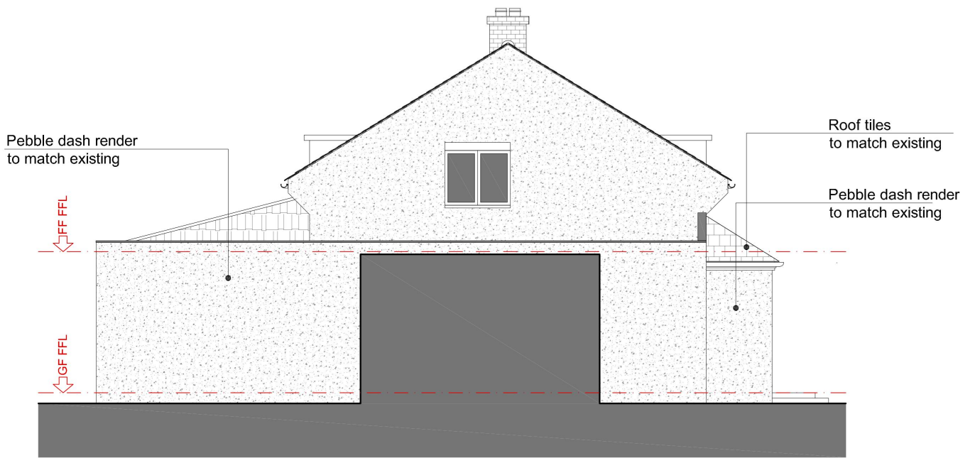
LHS ELEVATION
