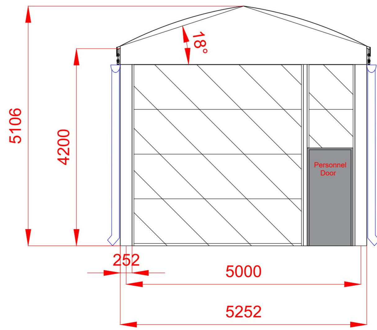
Elevation D
