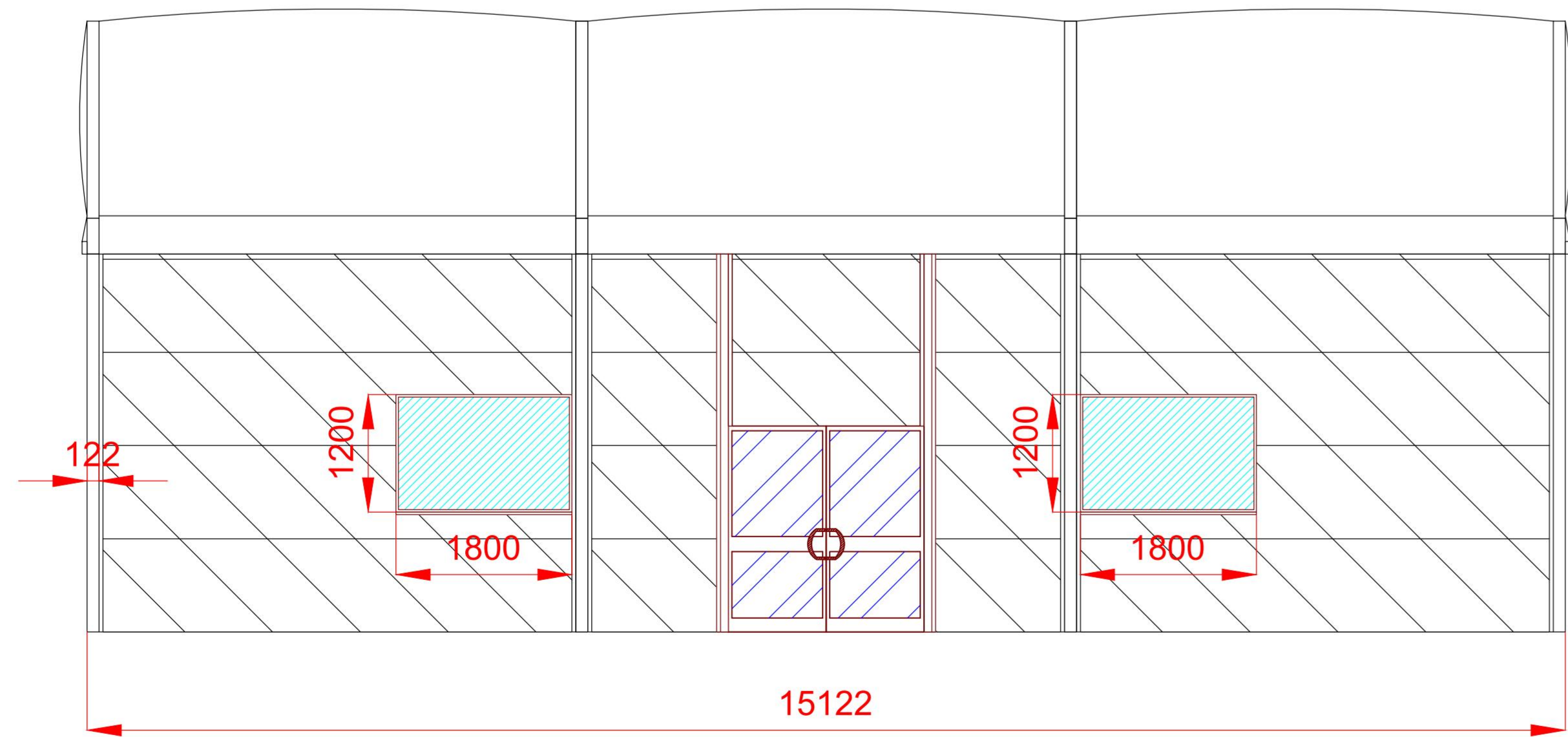
Elevation C
