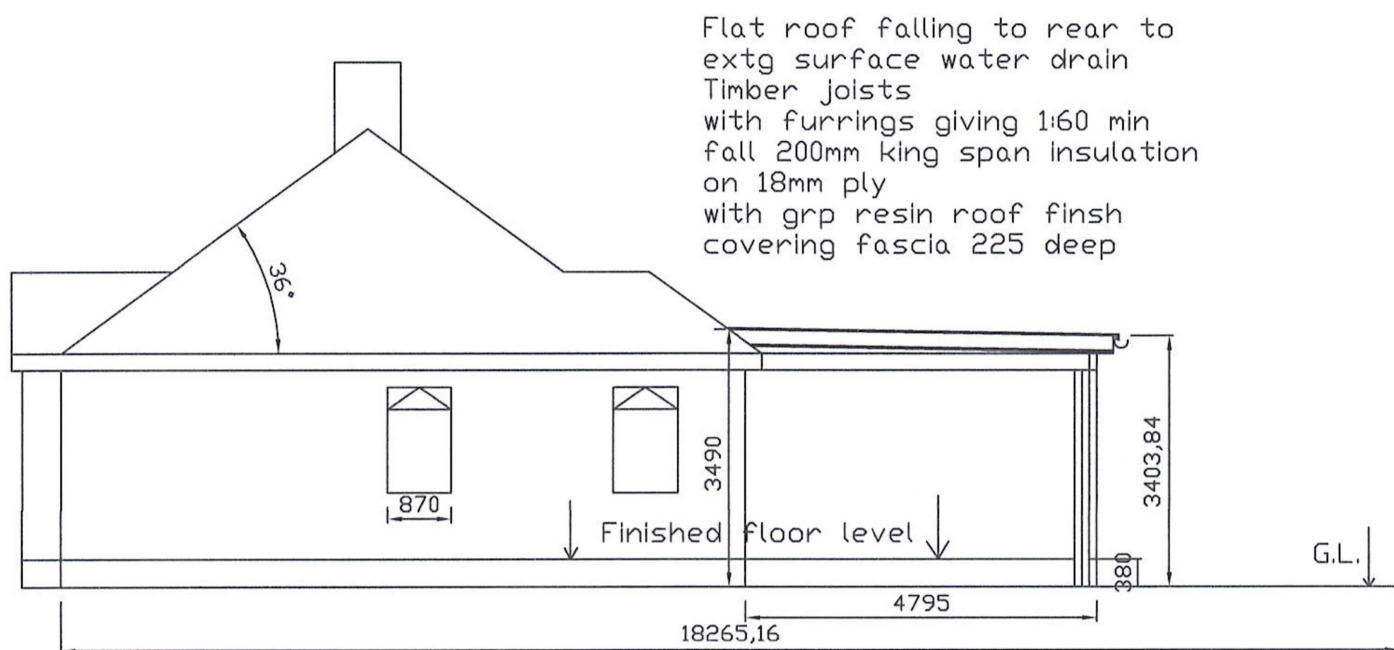
Extg side view of 288 Southend Arterial Road rendered with existing clear glazed windows
