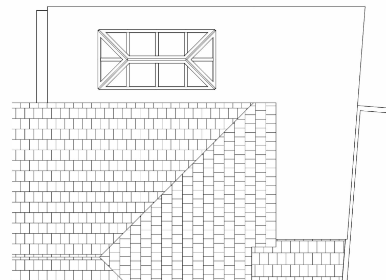
3 Proposed Roof Plan 1 : 100
