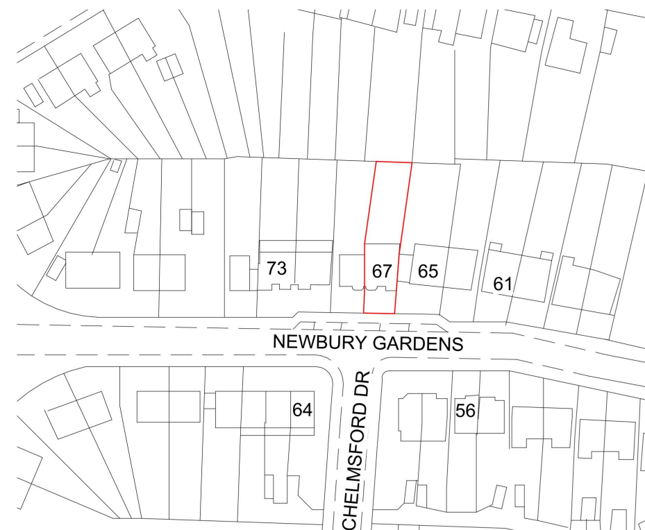
1 Site Location Plan 1 : 1250
