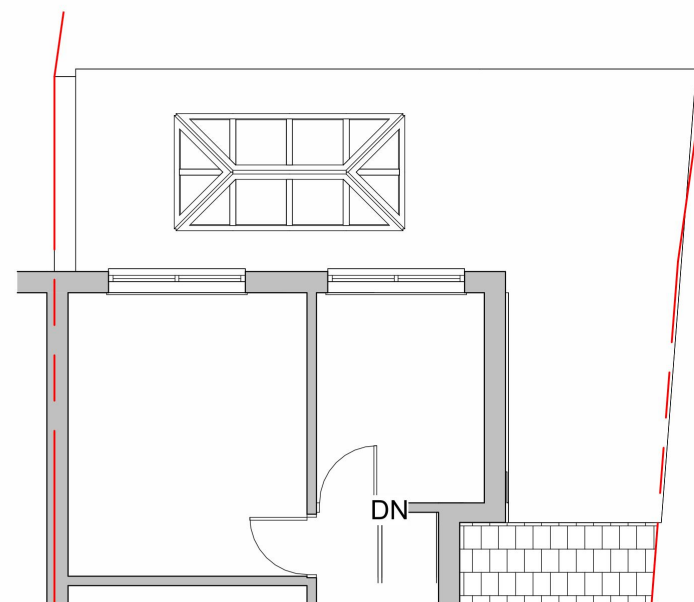
2 Proposed First Floor Plan 1 : 100
