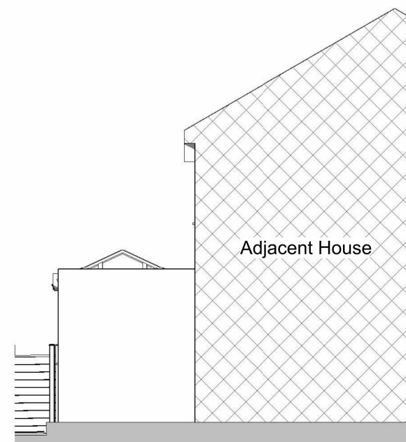
5 Existing North West Elevation 1 : 100
