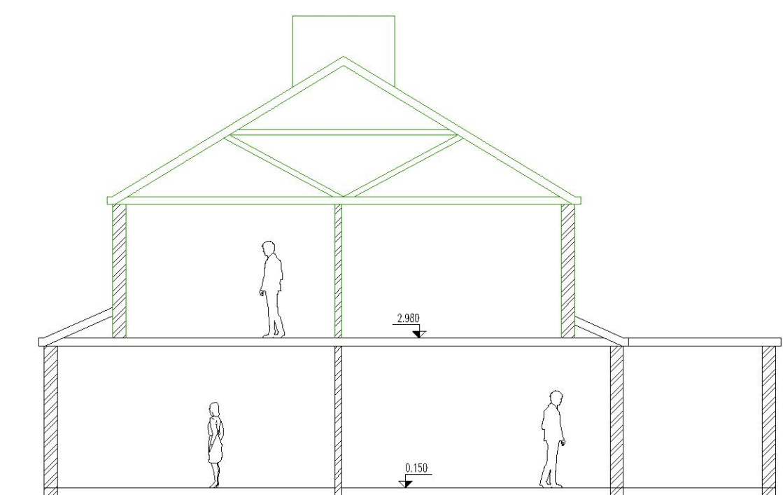
Proposed Flank Elevation SCALE 1/100
