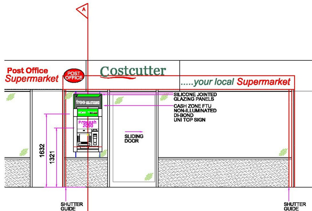
PROPOSED ELEVATION
