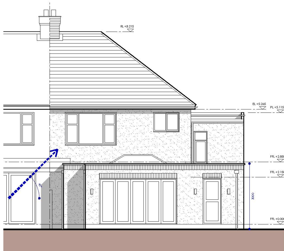
B - Proposed Rear Elevation - 1:100
