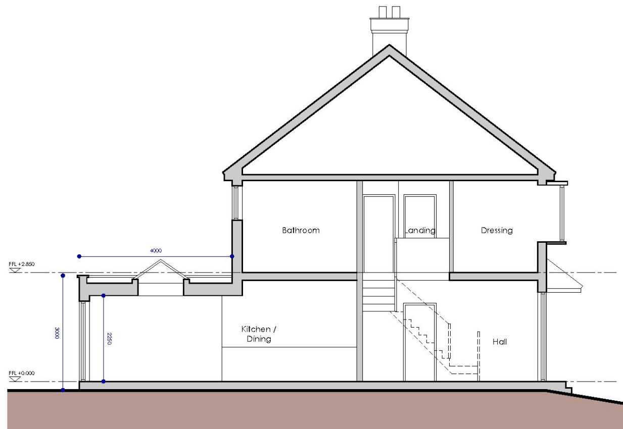
AA - Indicative Proposed Section - 1:100
