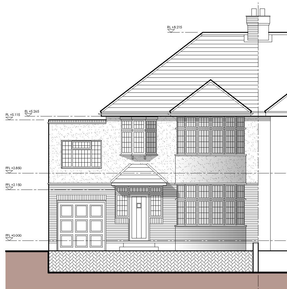
A - Proposed Front Elevation - 1:100
