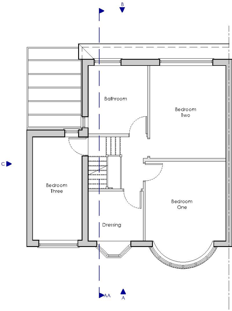
Existing First Floor - 1:100
