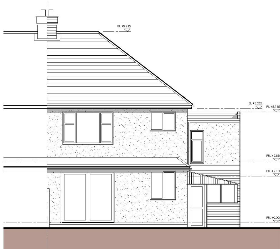
B - Existing Rear Elevation - 1:100
