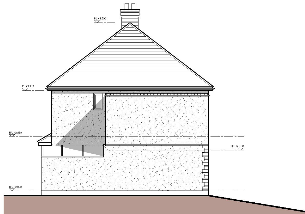
C - Existing Side Elevation - 1:100
