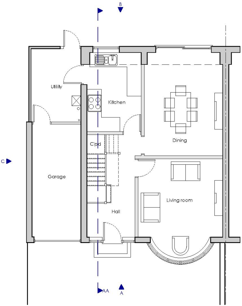
Existing Ground Floor - 1:100
