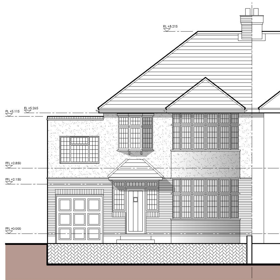
A - Existing Front Elevation - 1:100
