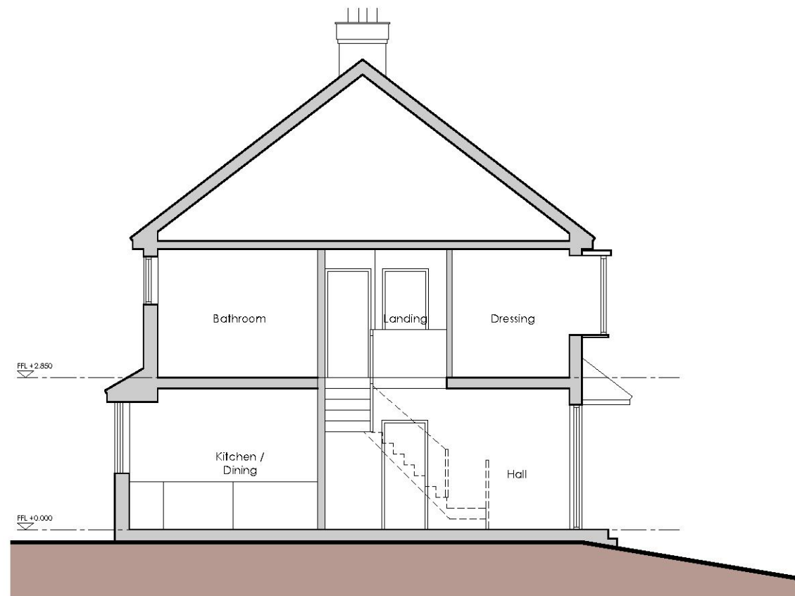
AA - Existing Section - 1:100
