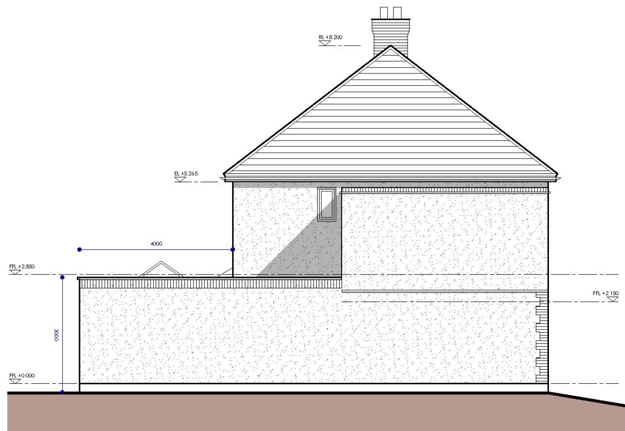
C - Proposed Side Elevation - 1:100
