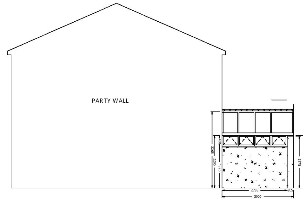
EXISTING LEFT ELEVATION
