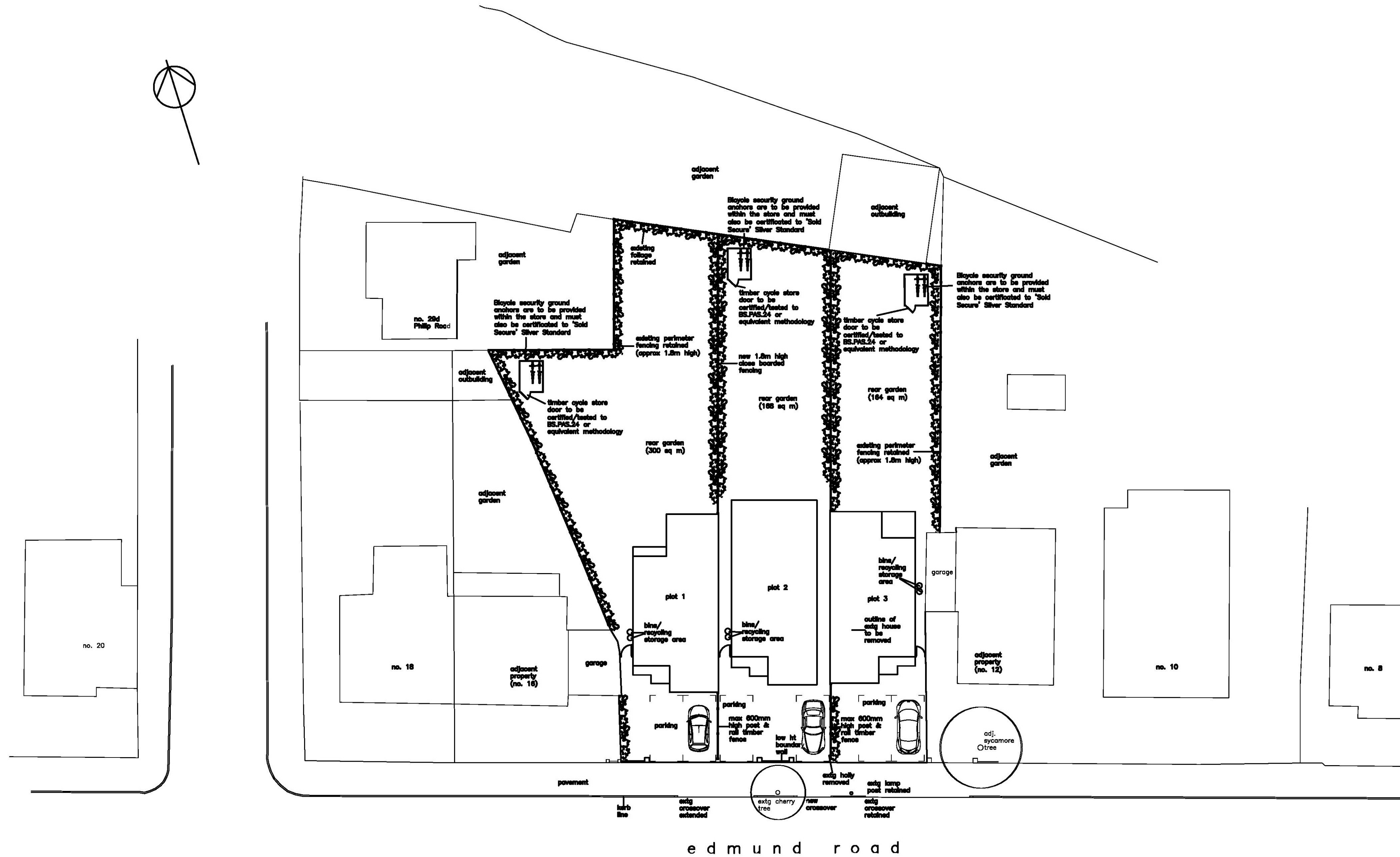
proposed block plan scale 1:200
